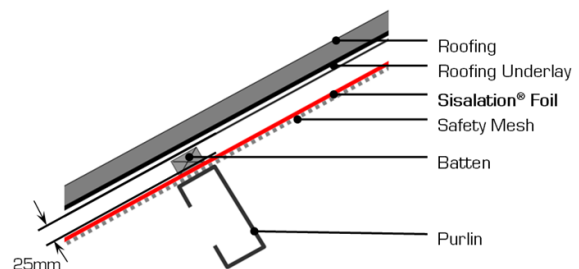
Typical Roof Installation
